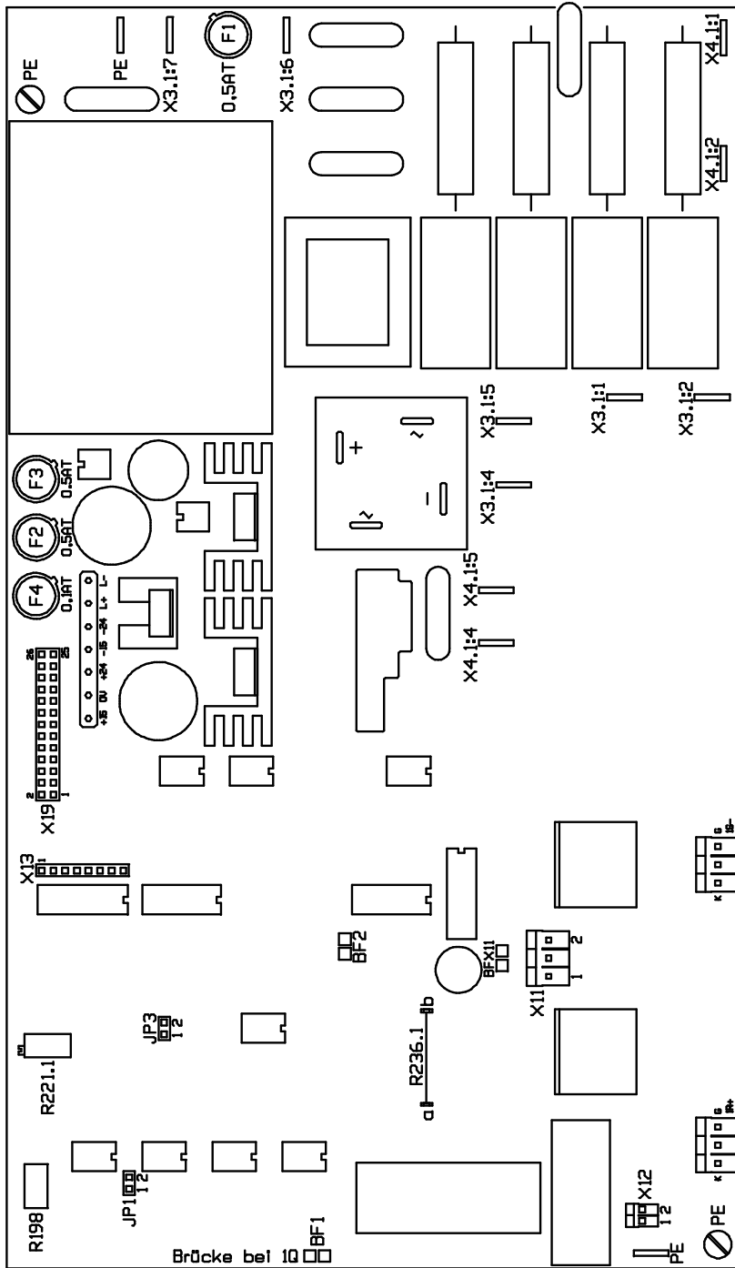
Open-loop controller circuit board GEE2 A0126xx
